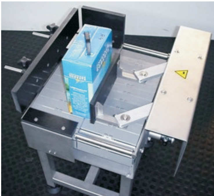
ZIMMERMANN-GRÄF-MÜLLER / D - ZELL Mosel reject conveyor 600mm for wine cartons 5-10ltr
