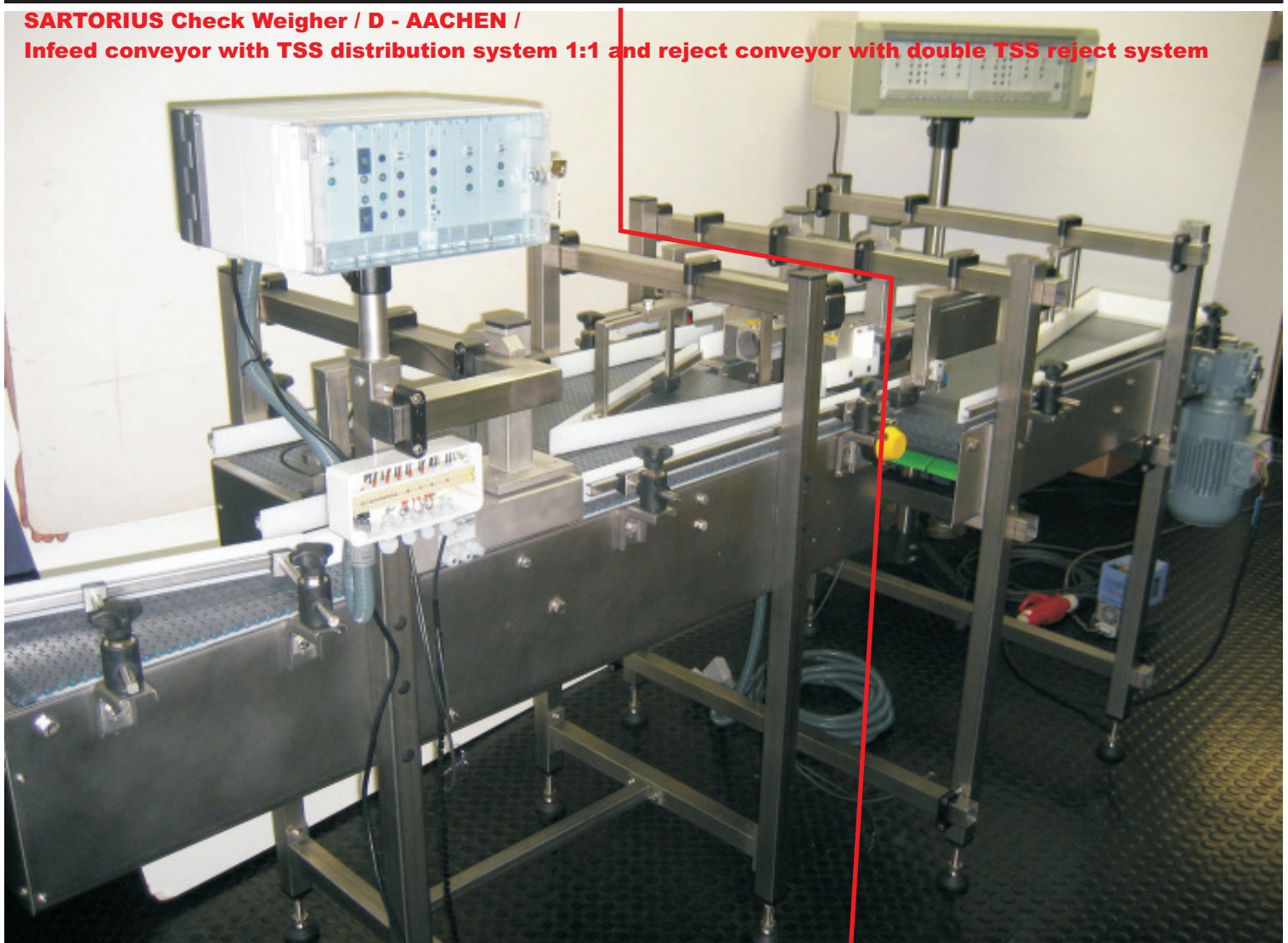
KOSMEPOL / PL - WARSCHAU / Vacuum Conveyor with noise-covered blowing motor for 180° bottle turning unit
