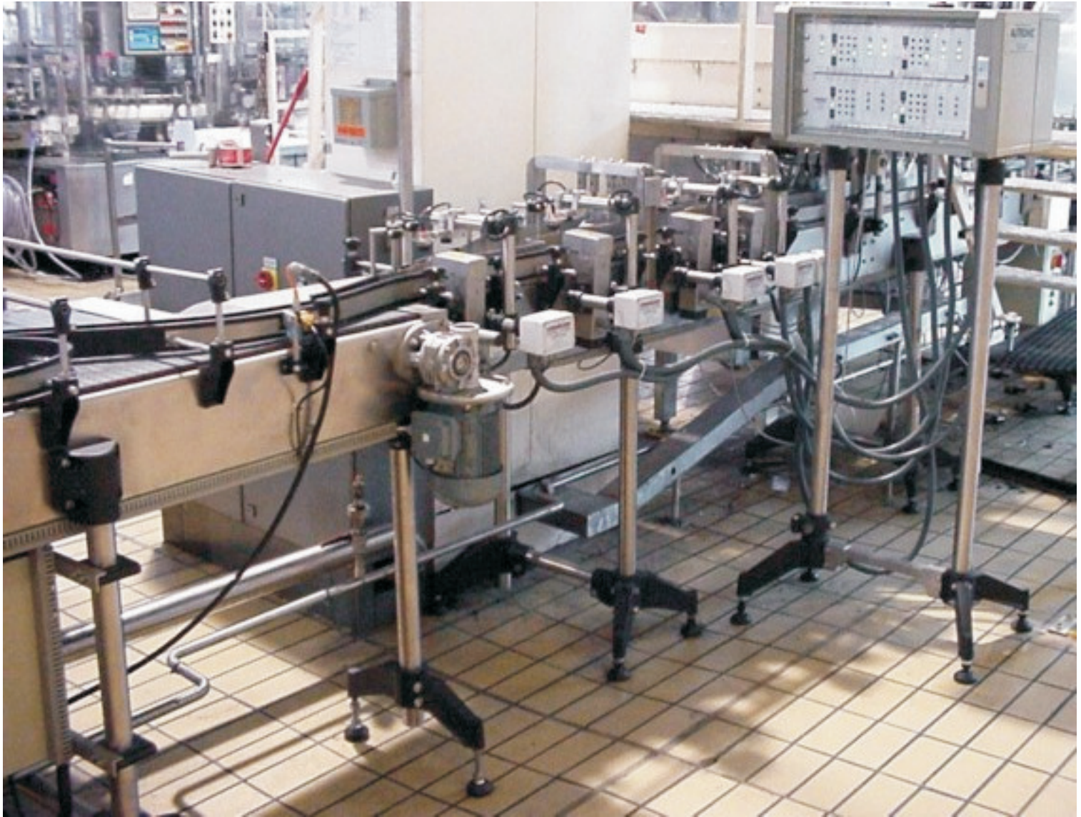
BAILEYS / IRL - DUBLIN production conveyor 6000mm with bottle distribution system 1 to 5 lanes
