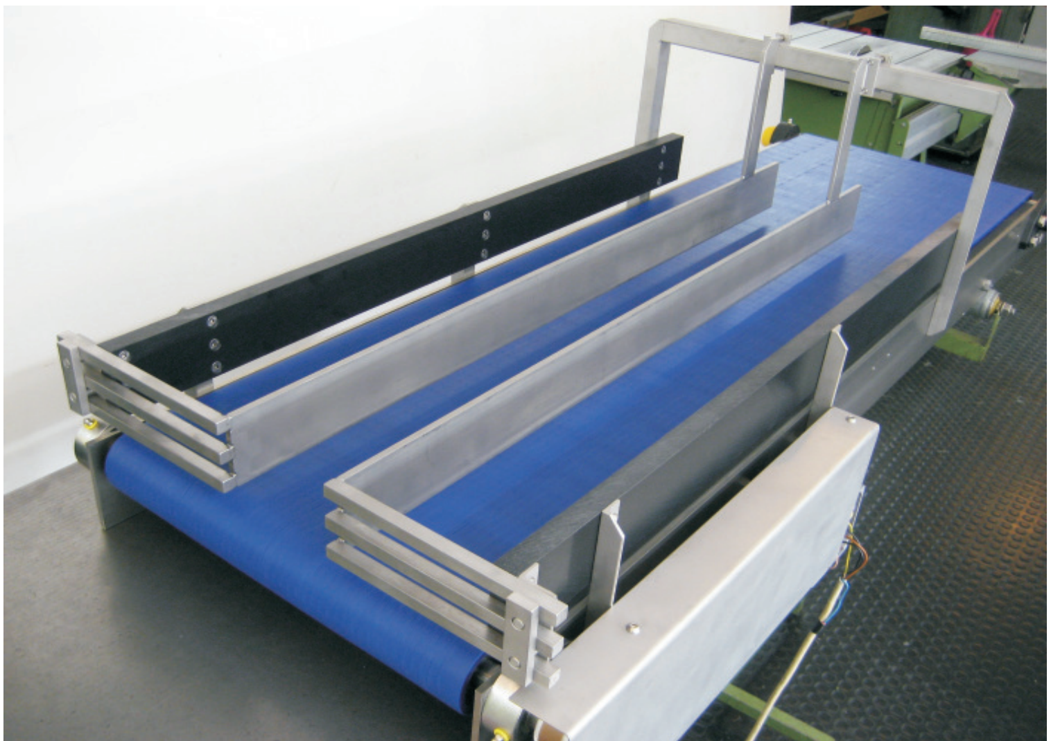
GLAXO SMITH KLINE / GB - / Reject conveyor after Mettler-Toledo-Garvens Check Weigher
