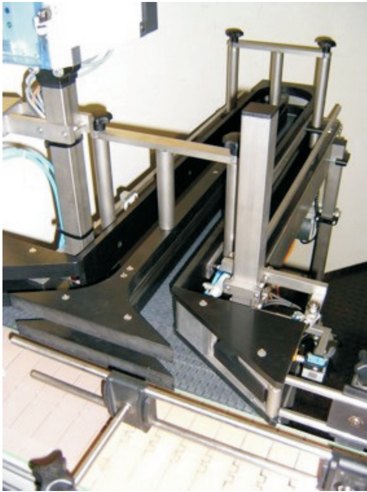
BODE CHEMIE / D - HAMBURG / accumulation conveyor with pneumatic infeed paddel and bottle flow monitoring
