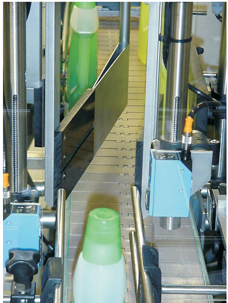
LUHNS GmbH / D - GREVEN / EMW - Reject System with luminescence label detection
